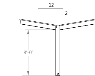
Minimum Clearance Height w/ MR Roof
