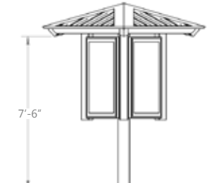
Minimum Clearance Height w/ MR Roof
