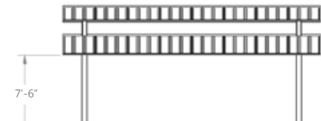
Minimum Clearance Height w/ MR Roof
