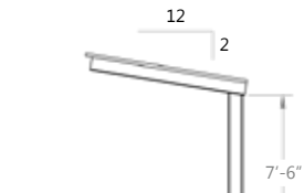
Minimum Clearance Height w/ MR Roof
