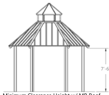
Minimum Clearance Height w/ MR Roof
