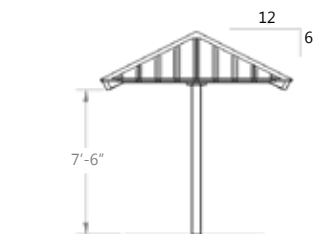
Minimum Clearance Height w/ MR Roof
